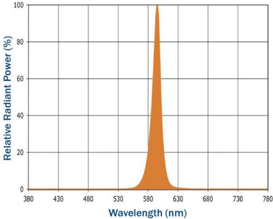
Spectral Chart - Amber LED
