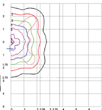
Distance in Units Of Mounting Height Values Based On 10 Foot Mounting Height 1/2 Maximum Candela Trace Shown As Dashed Curve (x) = Maximum Candela Point
