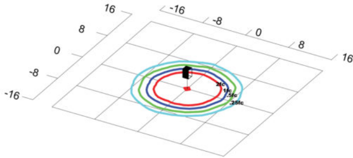
1 Footcandle Up to 6 Feet Away from the Bollard Light
