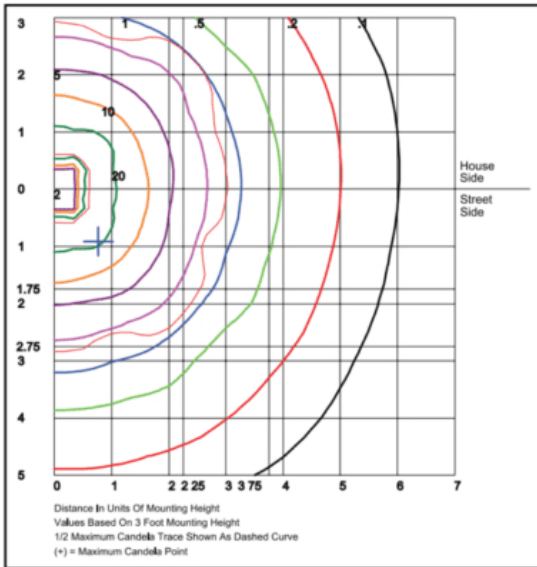
AF33XB2QF1X34U4KC & AF33XB2CQF1X34U4KC Type V, Clear Lens Grid in feet, Mounting Height = 3 ft.
