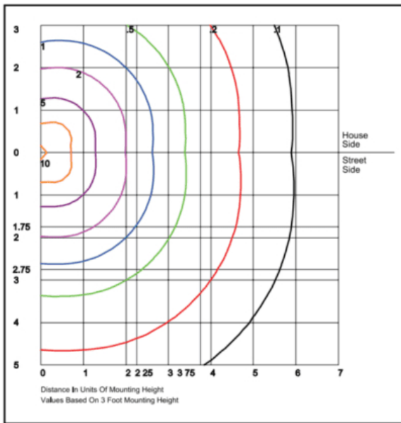
AF33XB2QF1X34U4KL & AF33XB2CQF1X34U4KL Type V, Opal Lens Grid in feet, Mounting Height = 3 ft.
